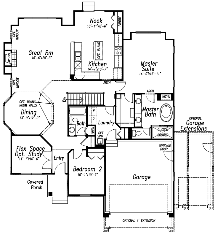
10' CEILING HEIGHT Main Level 1885 SQ FT
