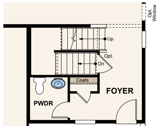
OPT. STAIRS AT BASEMENT
